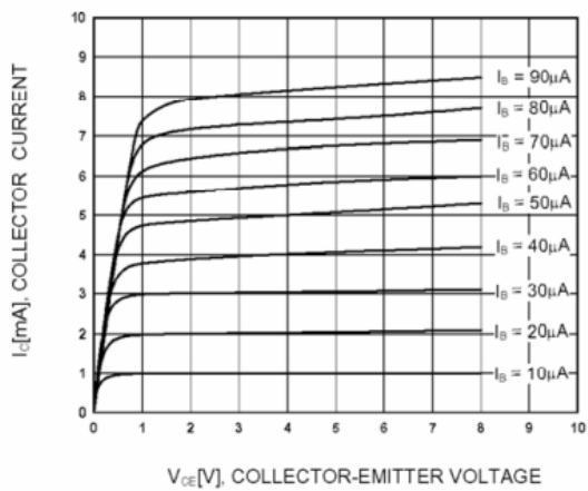
Static Characteristic
