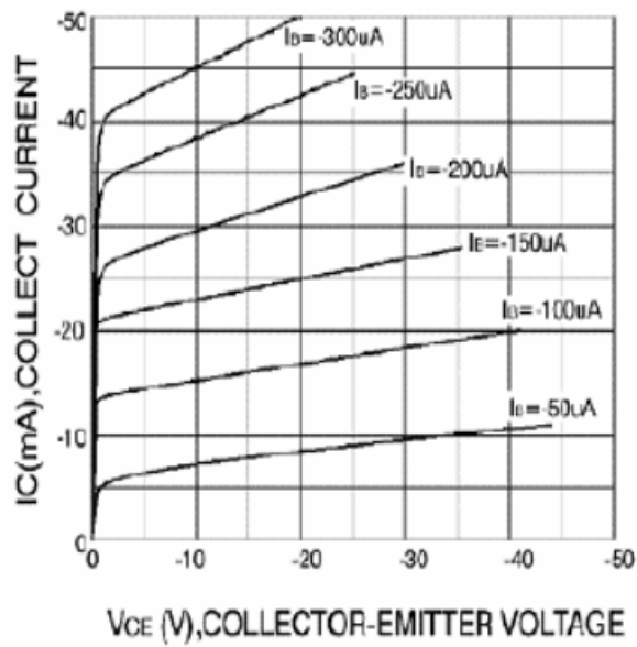
Static Characteristic
