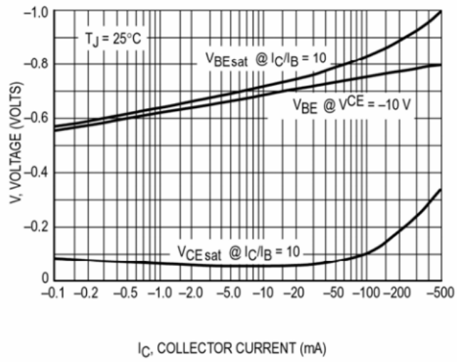
"On" Voltage
