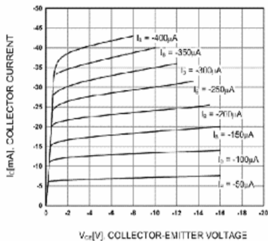
Static Characteristic
