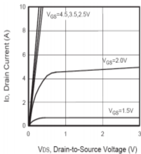
Figure3. Output Characteristics
